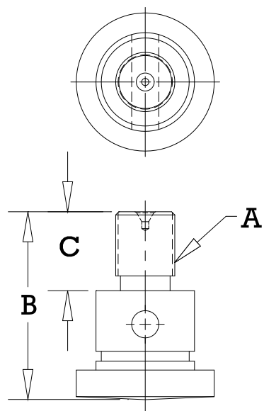
MALE ADAPTER *
